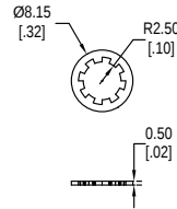
Lock Washer
