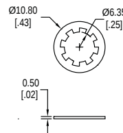
Lock Washer
